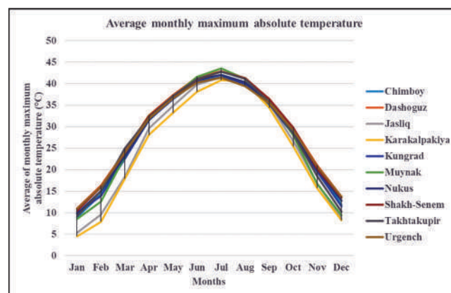
Figure 2. Average of monthly absolute maximum temperature ( ^{\circ}\text{C} ) during the recorded period of all the relative meteorostations.
